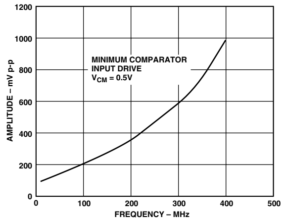
TPC 20. Comparator Toggle Voltage Requirement
