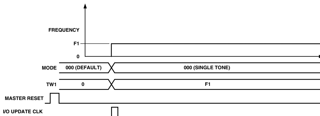
Figure 9. Default State to User-Defined Output Transition
