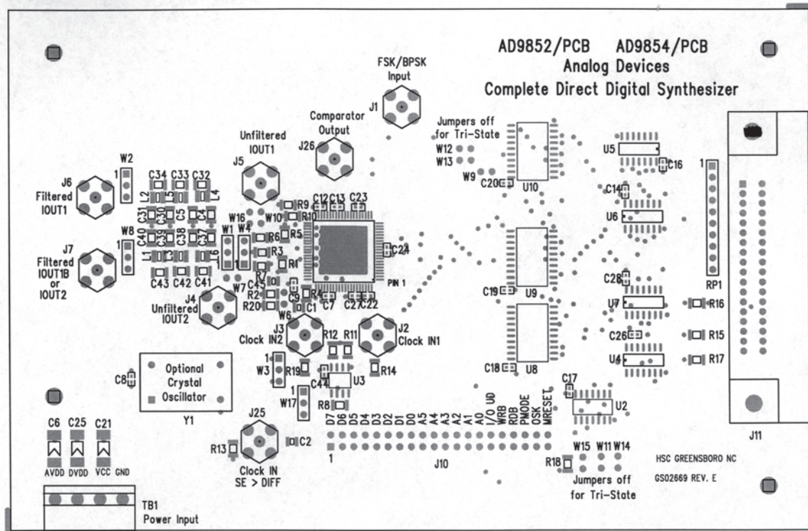
Figure 42. Assembly Drawing
