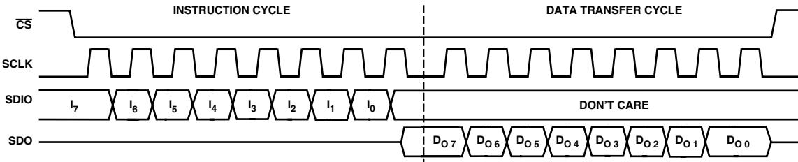
Figure 33. Three-Wire Serial Port Read Timing—Clock Stall Low
