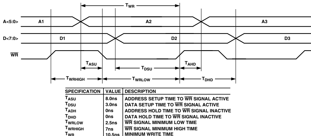
Figure 27. Parallel Port Write Timing Diagram
