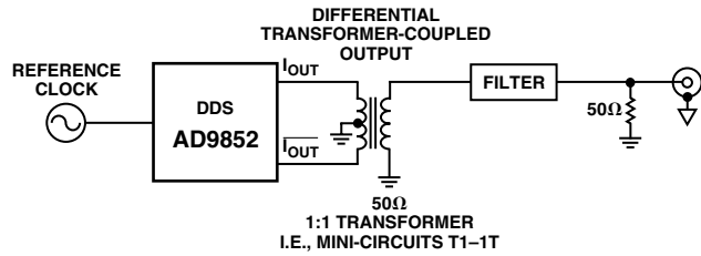
Figure 7. Differential Output Connection for Reduction of Common-Mode Signals
