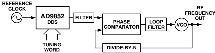
Figure 6. Agile High-Frequency Synthesizer
