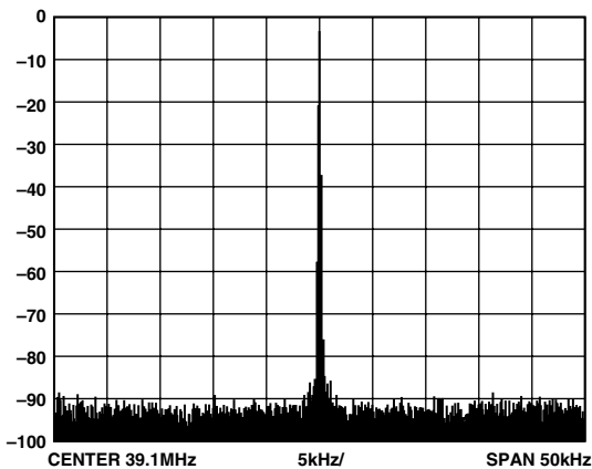
TPC 9. Narrowband SFDR, 39.1 MHz, 50 kHz BW, 100 MHz REFCLK with REFCLK Multiplier Bypassed
