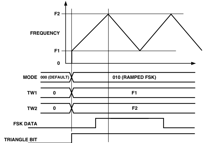
Figure 16. Automatic Linear Ramping Using the Triangle Bit
