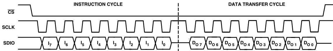
Figure 35. Two-Wire Serial Port Read Timing—Clock Stall High
