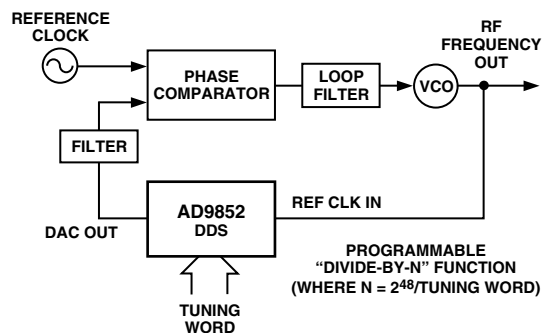
Figure 5. Programmable "Fractional Divide-by-N" Synthesizer
