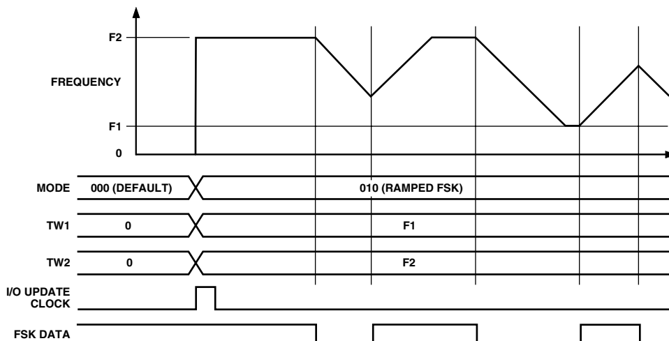
Figure 15. Effect of Premature Ramped FSK Data
