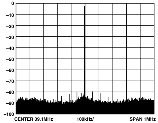
TPC 10. Narrowband SFDR, 39.1 MHz, 1 MHz BW, 30 MHz REFCLK with REFCLK Multiplier = 10x
