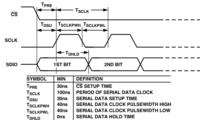
Figure 30. Timing Diagram for Data Write to AD9852
