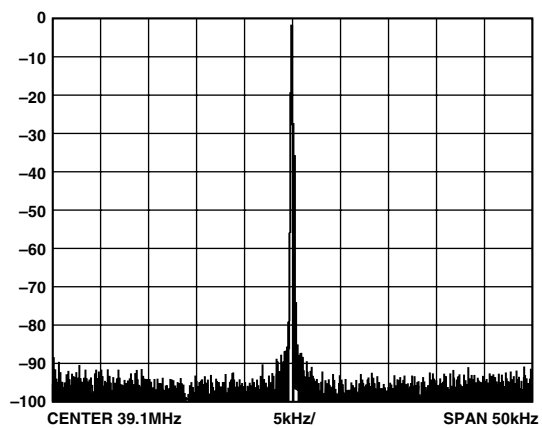
TPC 14. Narrowband SFDR, 39.1 MHz, 50 kHz BW, 200 MHz REFCLK with REFCLK Multiplier Bypassed
