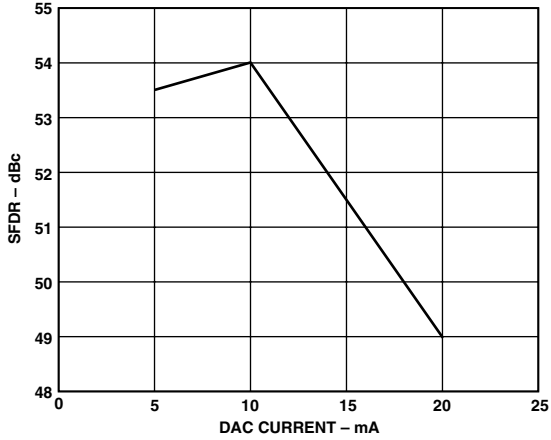
TPC 16. SFDR vs. DAC Current, 59.1 A_{OUT} , 300 MHz REFCLK with REFCLK Multiplier Bypassed
