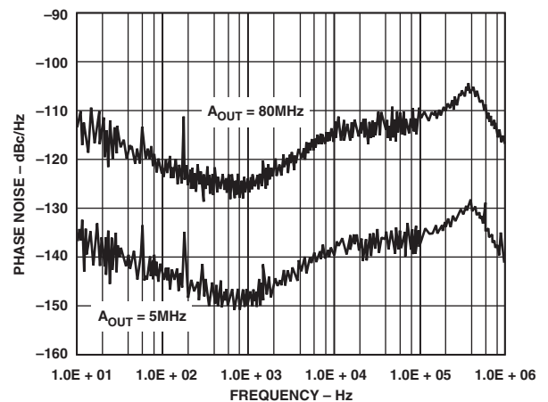
TPC 15b. Residual Phase Noise, 30 MHz REFCLK with REFCLK Multiplier = 10×
