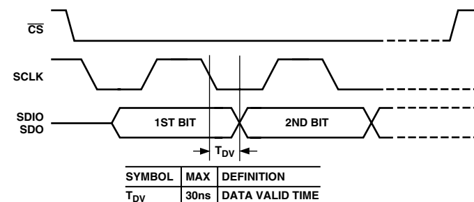
Figure 31. Timing Diagram for Read from AD9852
