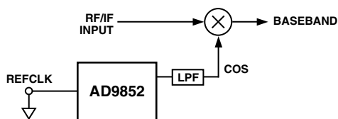
Figure 2. Synthesized L.O. Application for the AD9852
