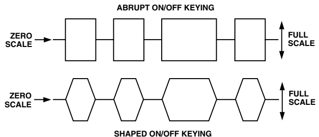
Figure 23. Shaped On/Off Keying
