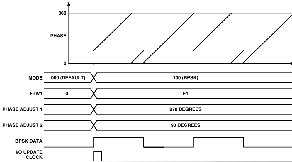
Figure 22. BPSK Mode
