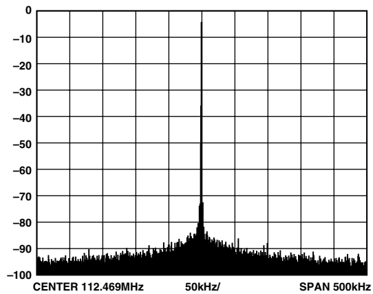
TPC 13. A slight change in tuning word yields dramatically better results. 112.469 MHz with all spurs shifted out-of-band. REFCLK is 300 MHz.
