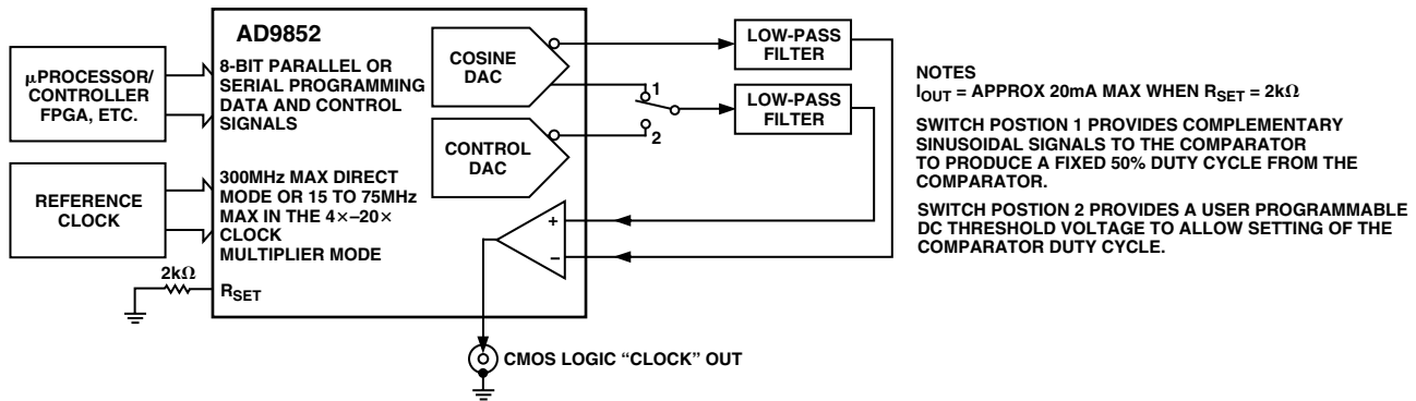
Figure 8. Frequency Agile Clock Generator Applications for the AD9852
