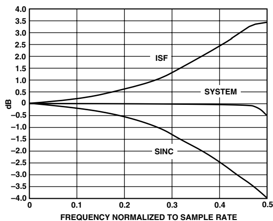
Figure 25. Inverse SINC Filter Response
