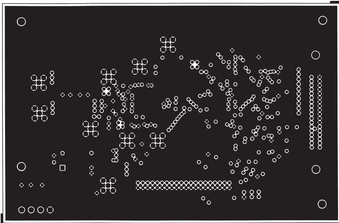
Figure 45. Power Plane Layer, Layer 3
