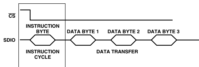
Figure 28. Using SDIO as a Read/Write Transfer
