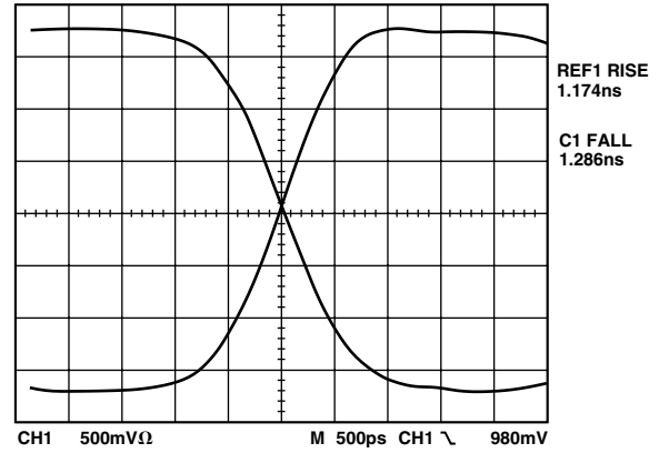
TPC 19. Comparator Rise/Fall Times
