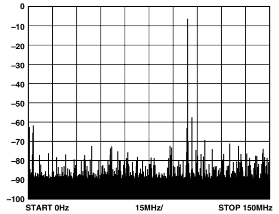
TPC 5. Wideband SFDR, 99.1 MHz
