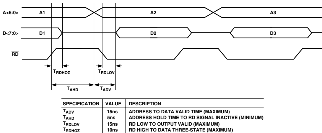
Figure 26. Parallel Port Read Timing Diagram
