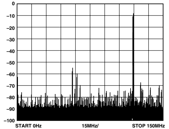
TPC 6. Wideband SFDR, 119.1 MHz
