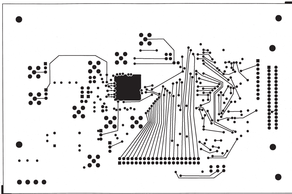
Figure 46. Bottom Routing Layer, Layer 4
