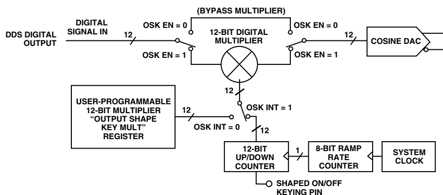
Figure 24. Block Diagram of the Digital Multiplier Section Responsible for Shaped Keying Function
