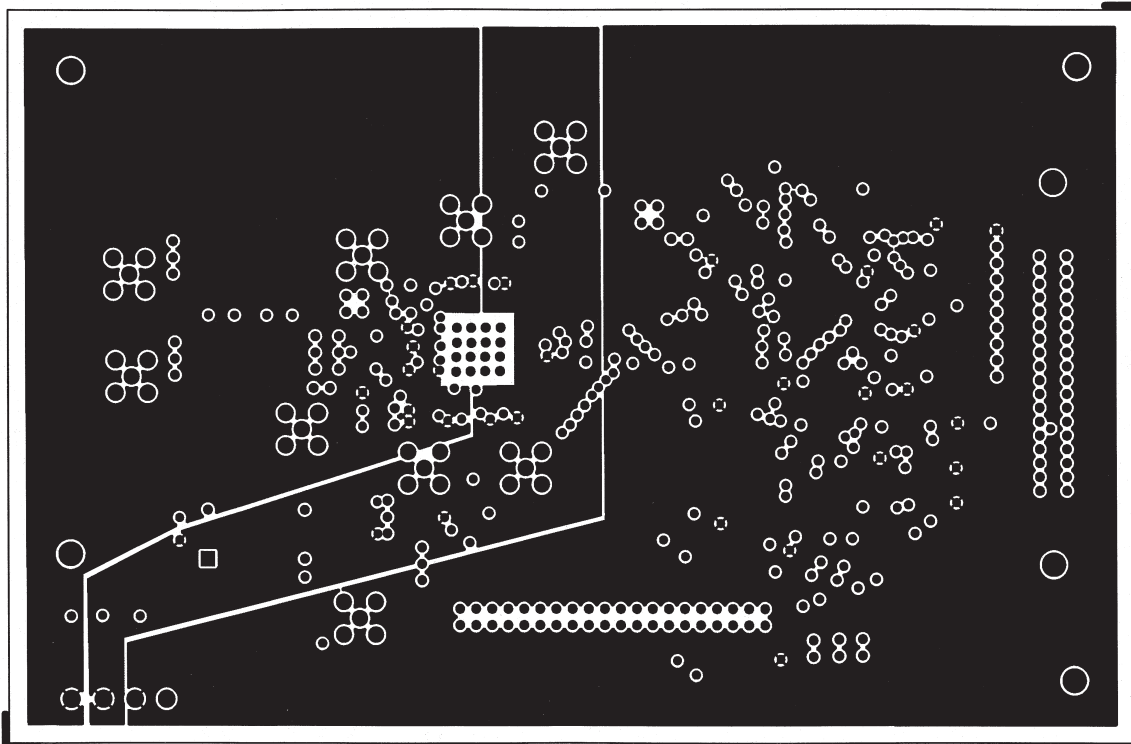
Figure 44. Ground Plane Layer, Layer 2
