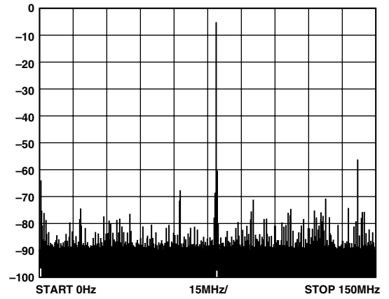
TPC 4. Wideband SFDR, 79.1 MHz
